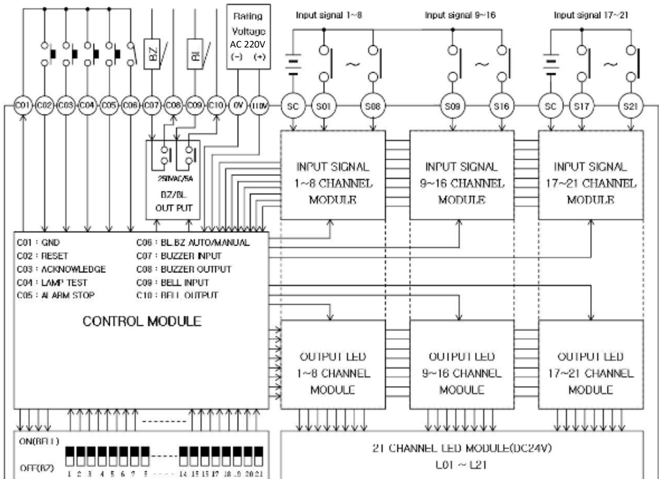
Inside Circuit Diagram(21CH)
