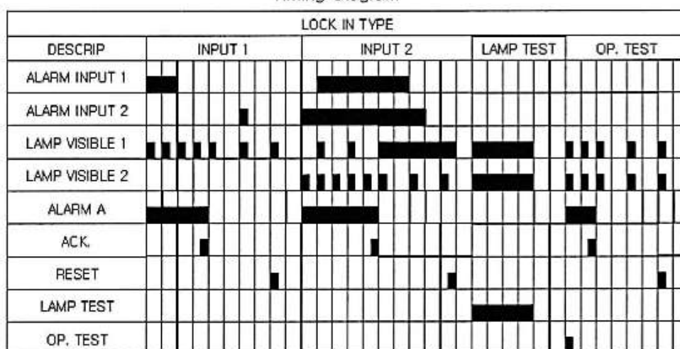
Timing Diagram
